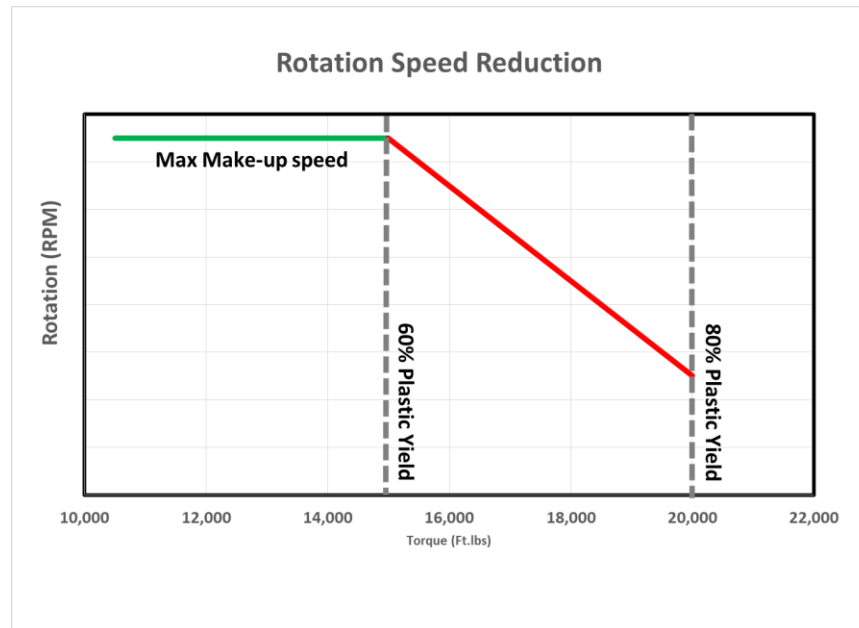
FIGURE Rotation limit based on running torque
